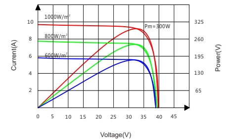
Current-Voltage&Power-Voltage Curve(300W)
